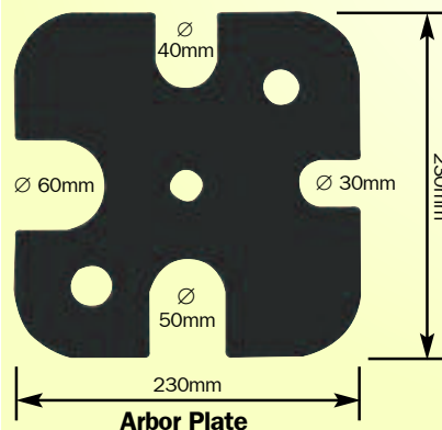
Arbor Plate
